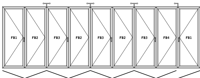
P900D1 (8+1)
