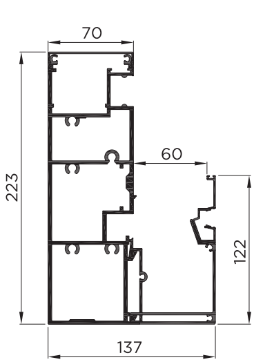
SET CHANNEL ASSEMBLY
