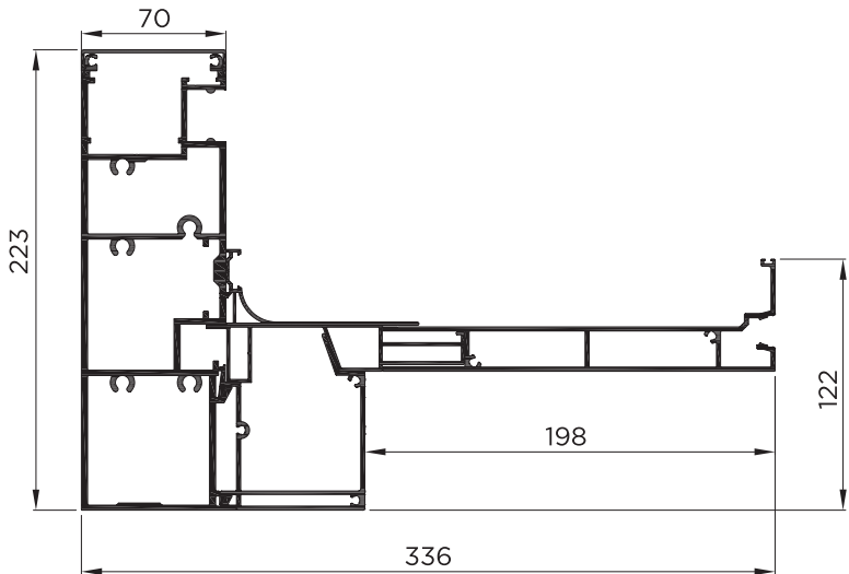
SET COMPENSATOR ASSEMBLY
