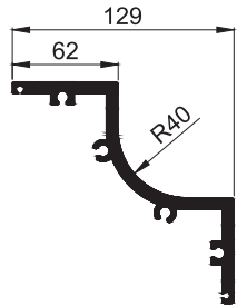
ANGULAR REINFORCEMENT
