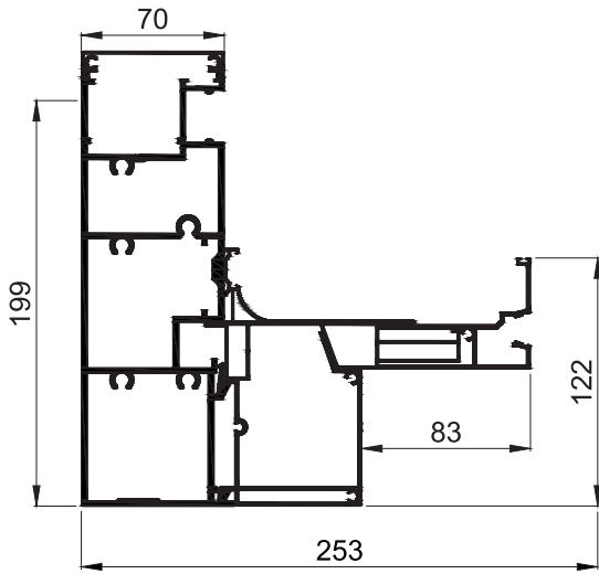
UPRIGHT-COMPENSATOR ASSEMBLY WITH REDUCTION
